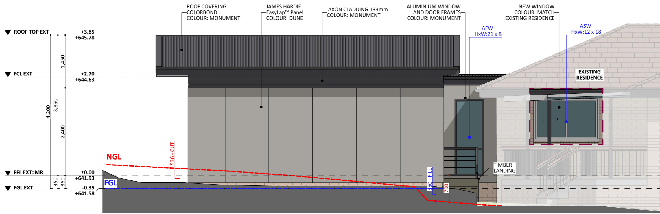
SOUTH ELEV.
