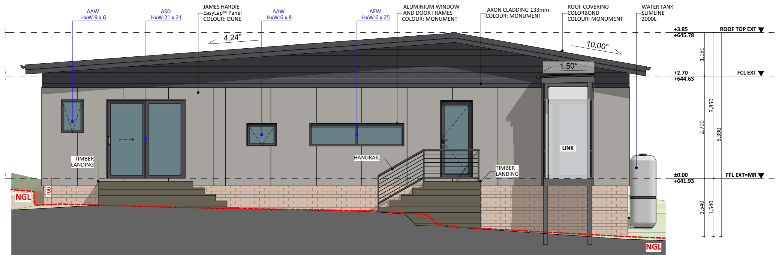
EAST ELEV.
