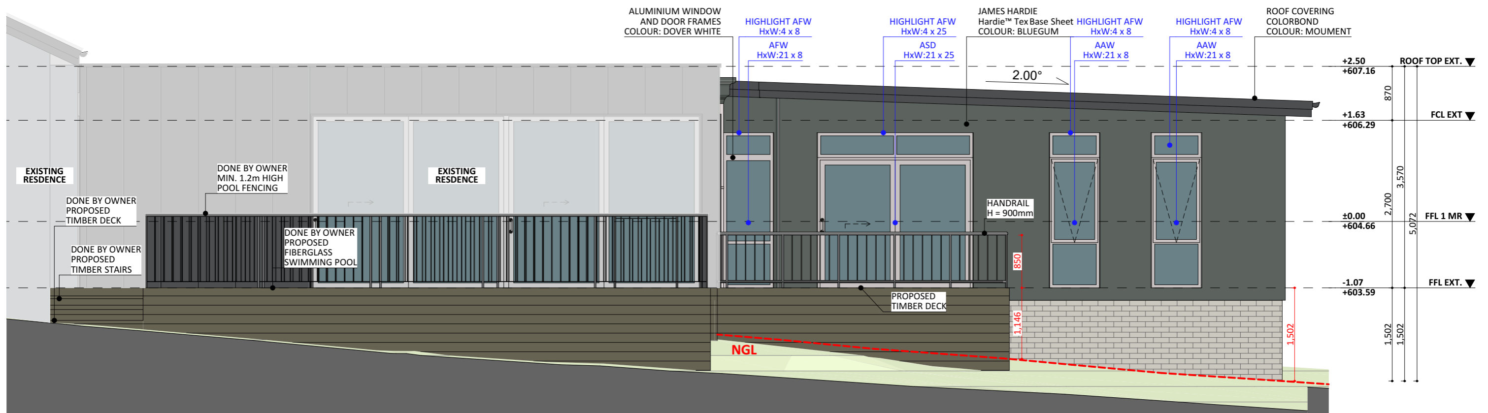
NORTH ELEV.
