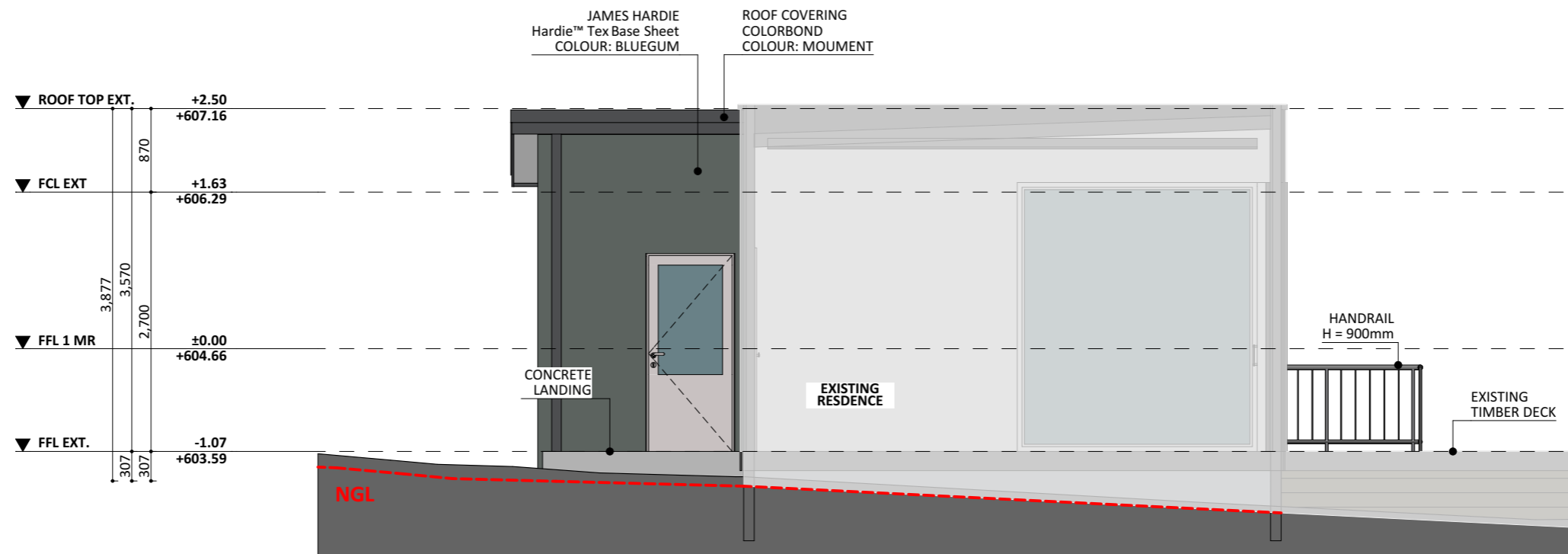
EAST ELEV.
