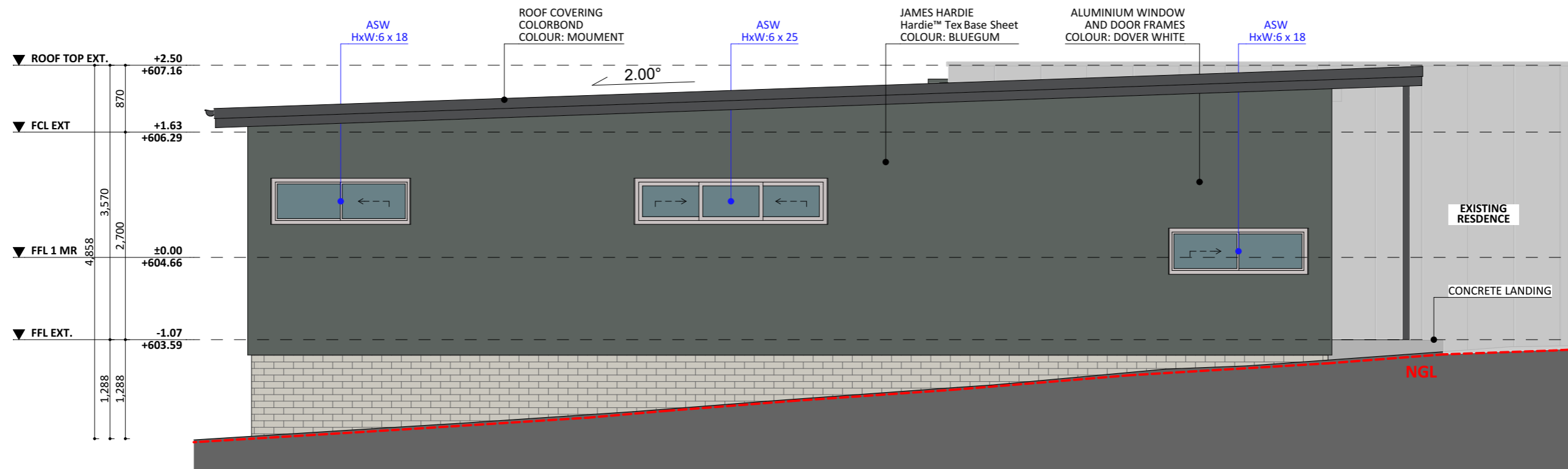
SOUTH ELEV.
