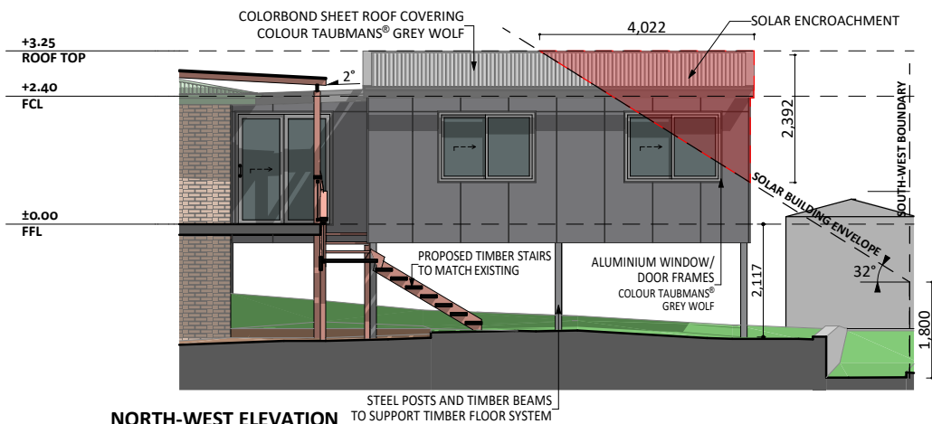
NORTH-WEST ELEVATION
