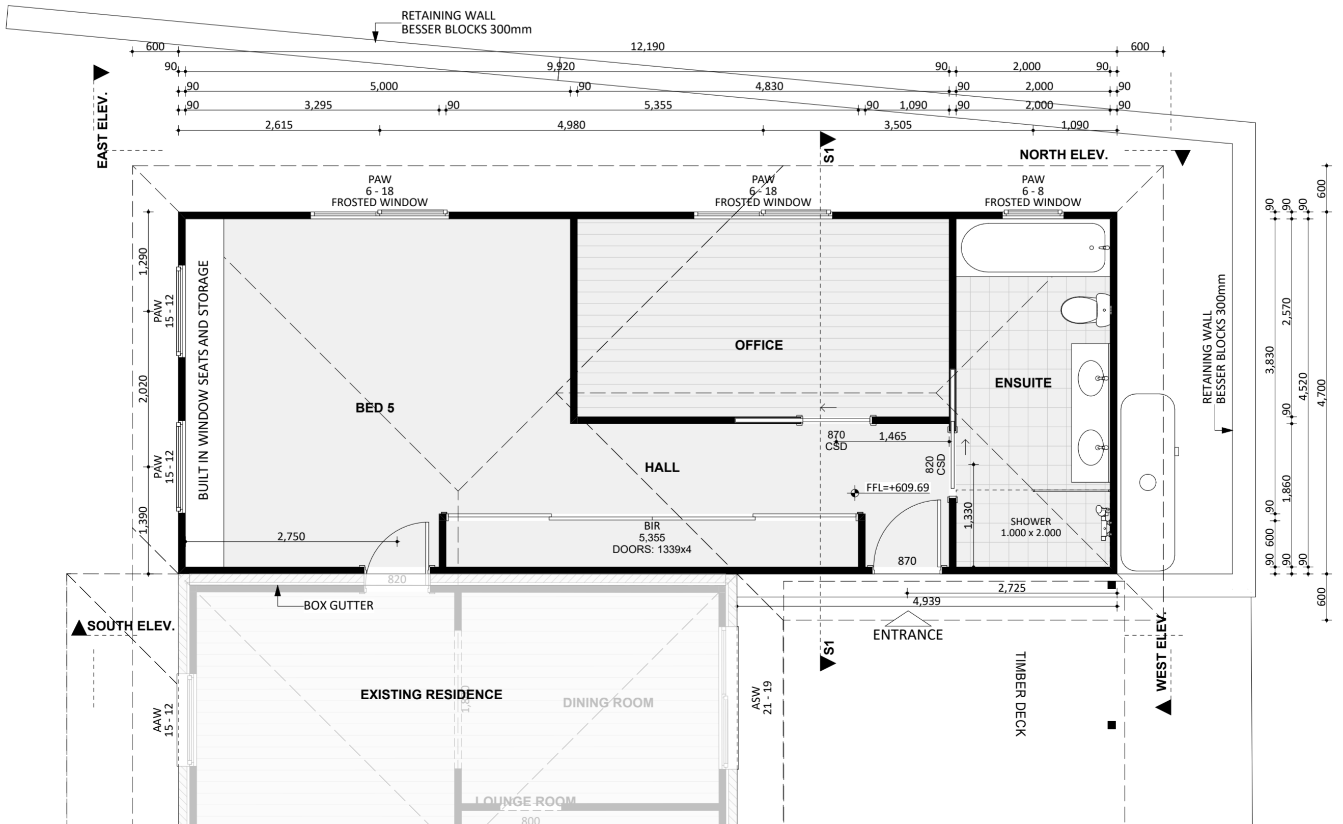
FIRST FLOOR
