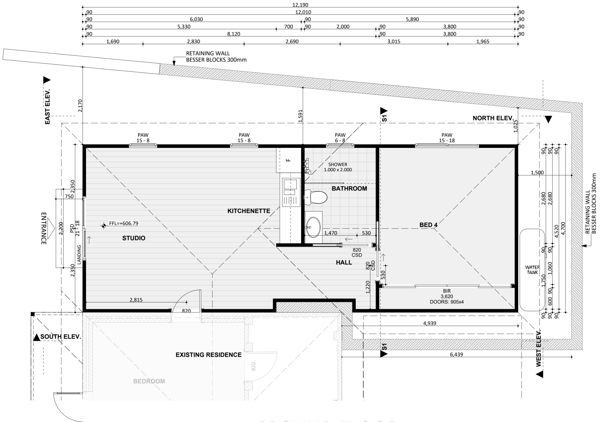
GROUND FLOOR
