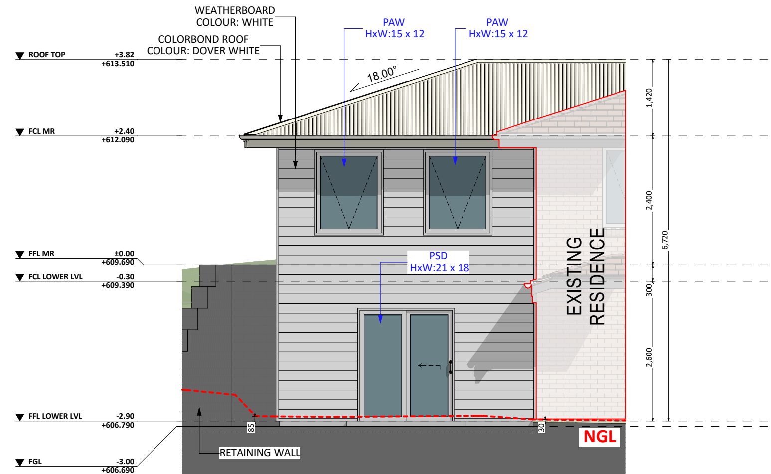
S7 EAST ELEV.
