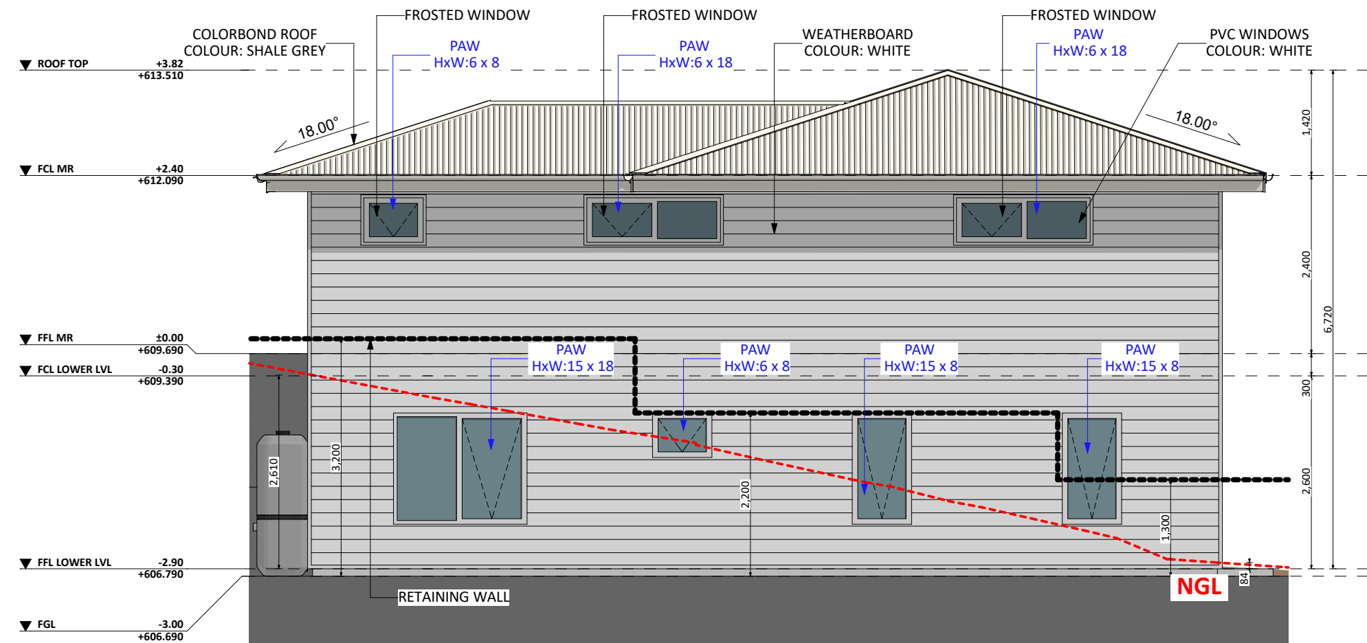
S4 NORTH ELEV.
