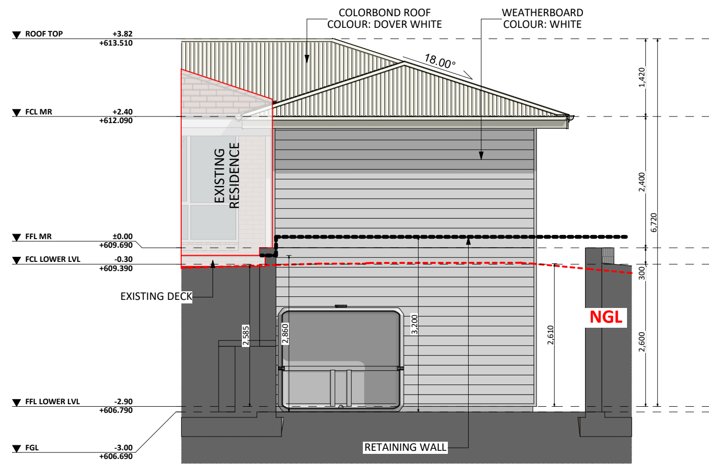
S5 WEST ELEV.
