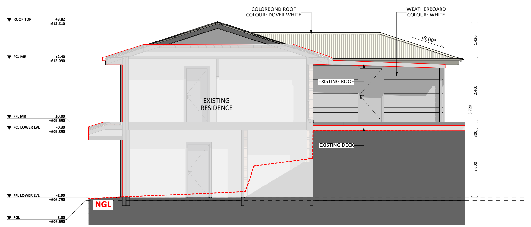
S6 SOUTH ELEV.
