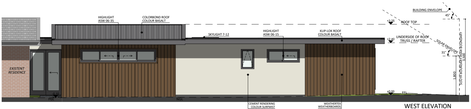
WEST ELEVATION
