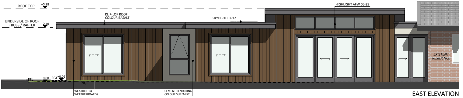
EAST ELEVATION
