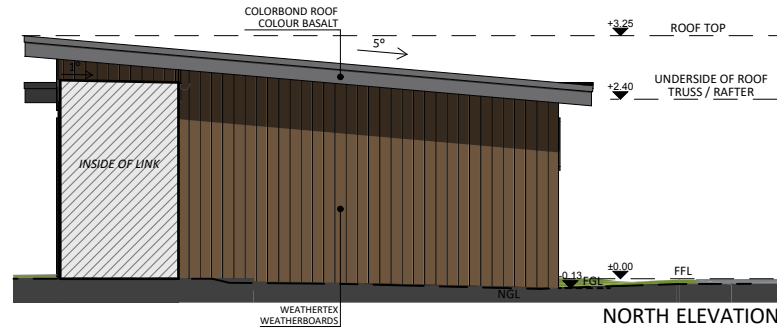
NORTH ELEVATION
