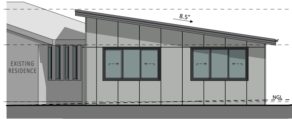
WEST ELEVATION
