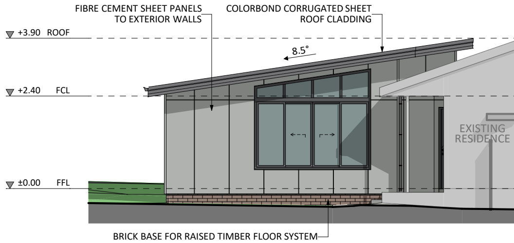
EAST ELEVATION
