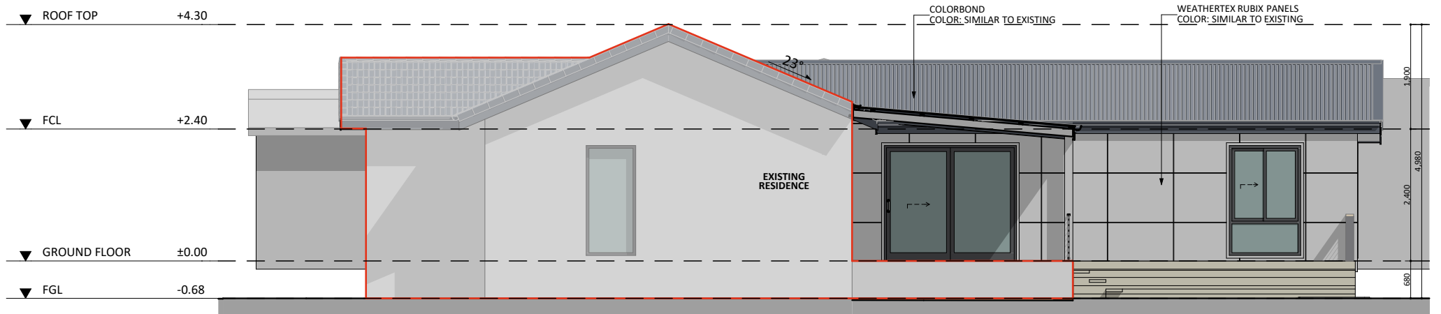
NORTH-WEST ELEVATION
