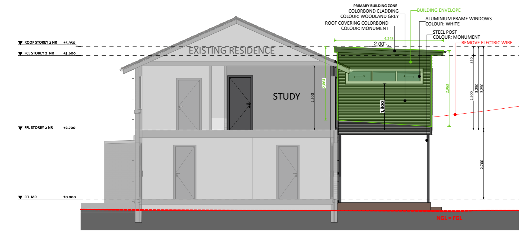
ELEVATION 03
