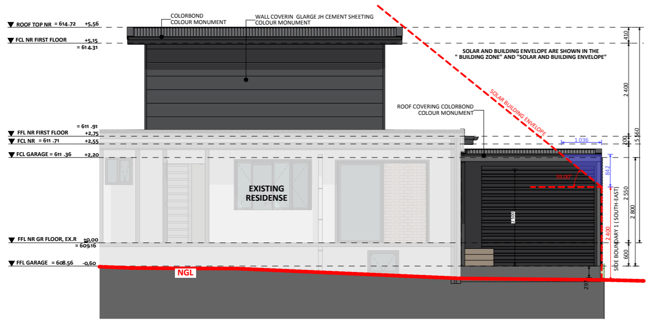
ELEVATION 03
