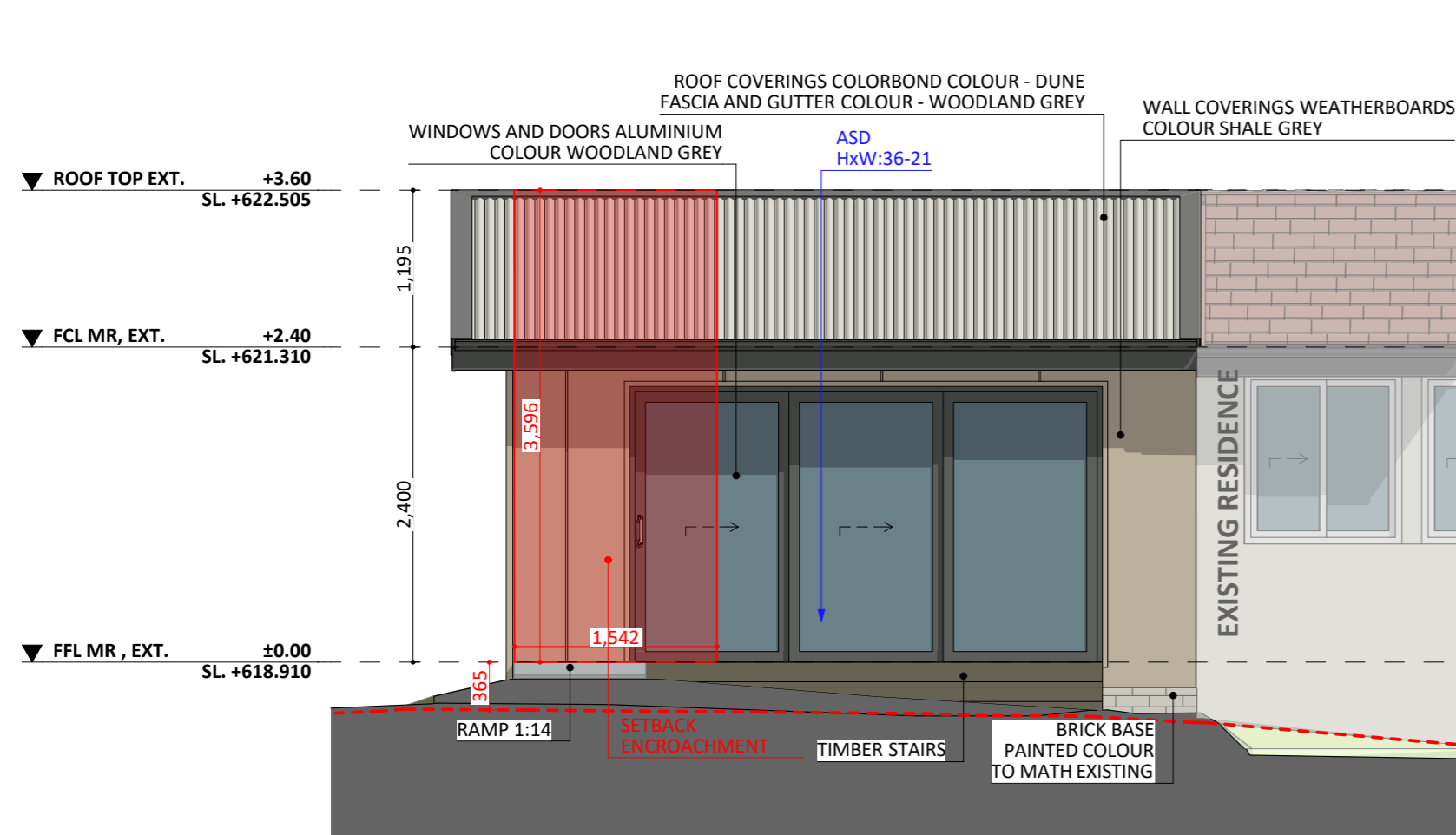
NORTH - EAST ELEVATION - CL 1168
