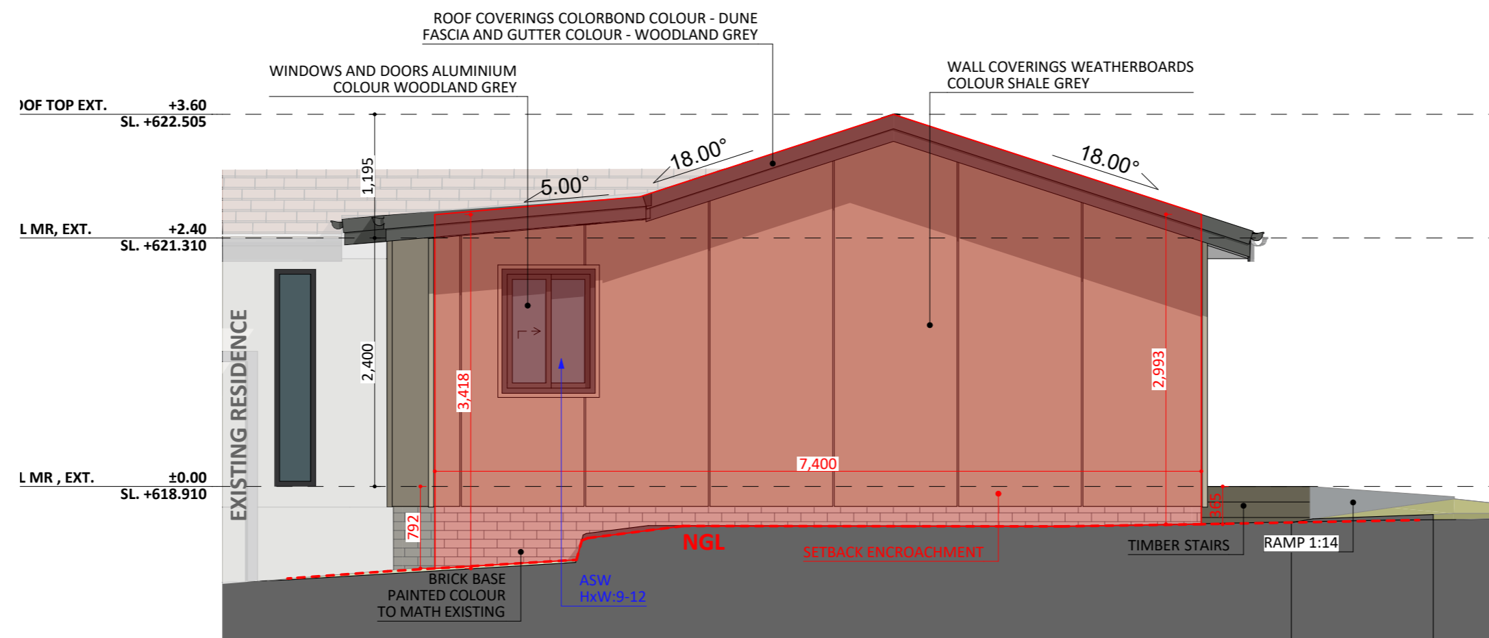
SOUTH - EAST ELEVATION - CL 1168
