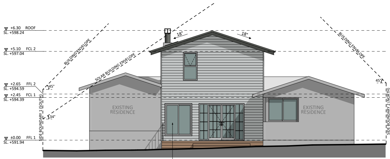
EAST ELEVATION
