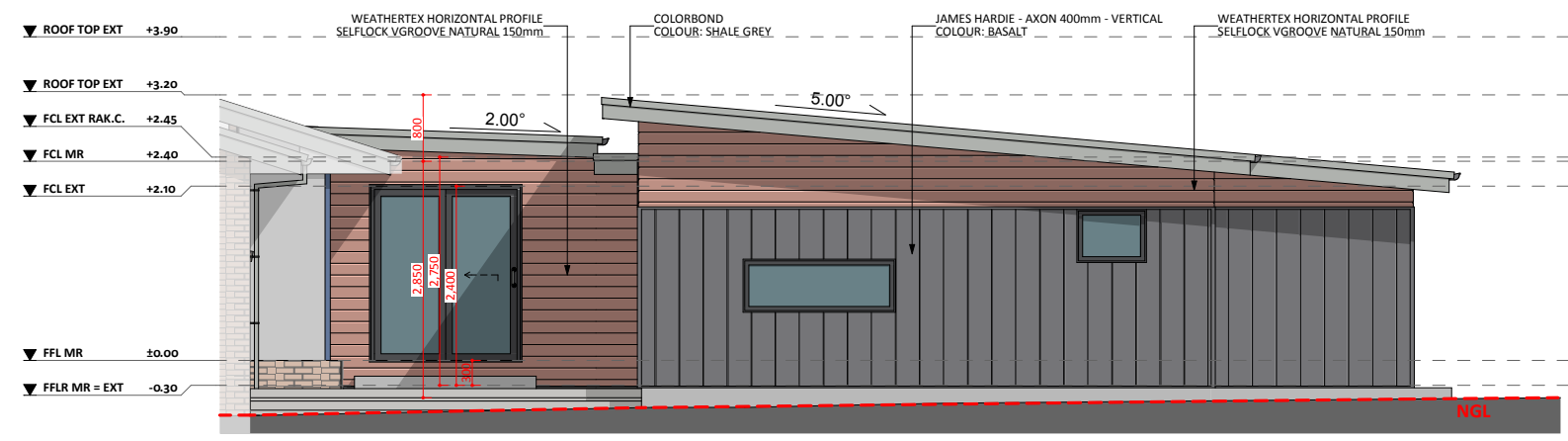
WEST ELEV.
