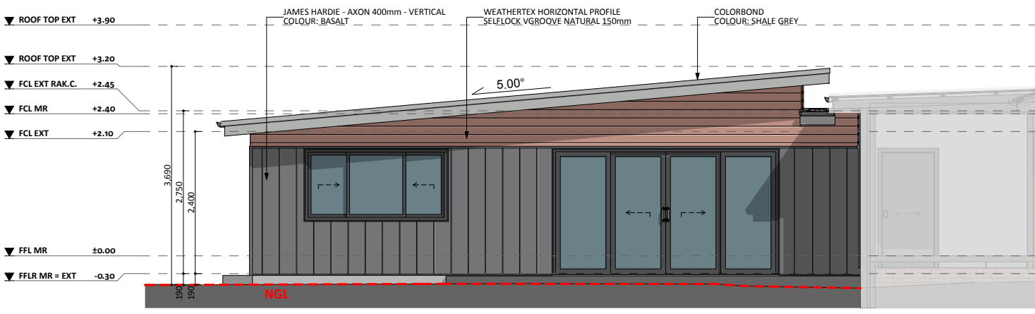
EAST ELEV.
