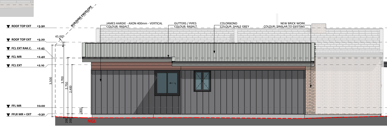
SOUTH ELEV.
