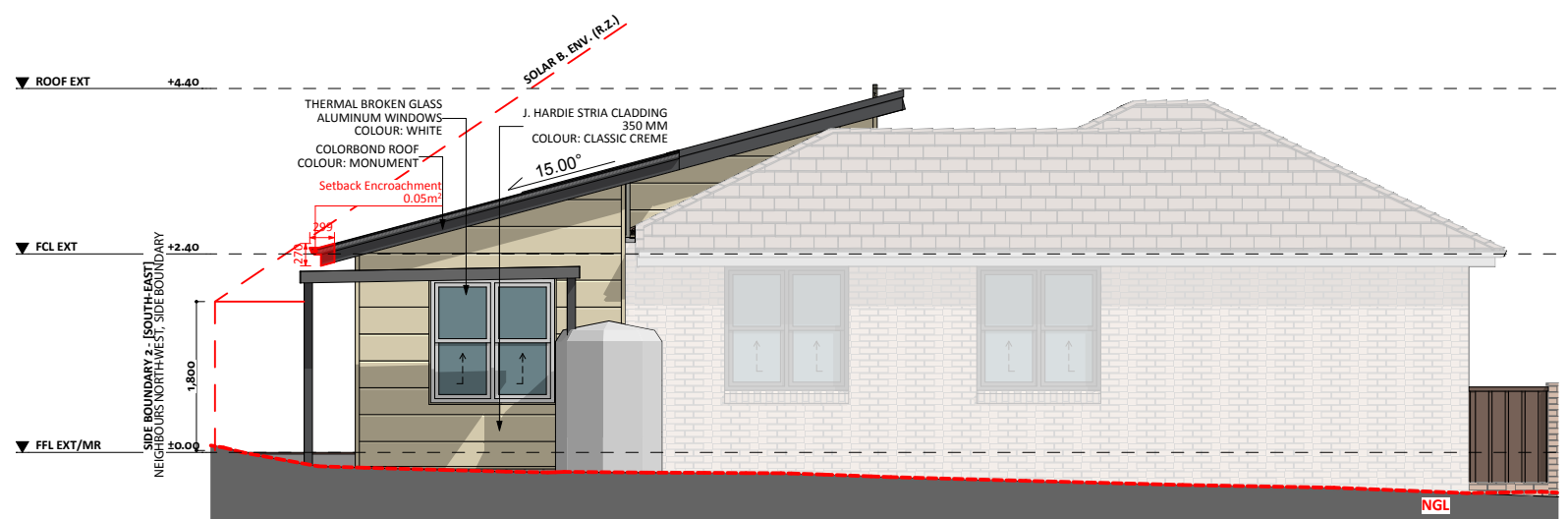
ELEVATION 03
