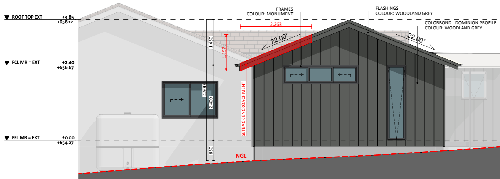
ELEVATION 03
