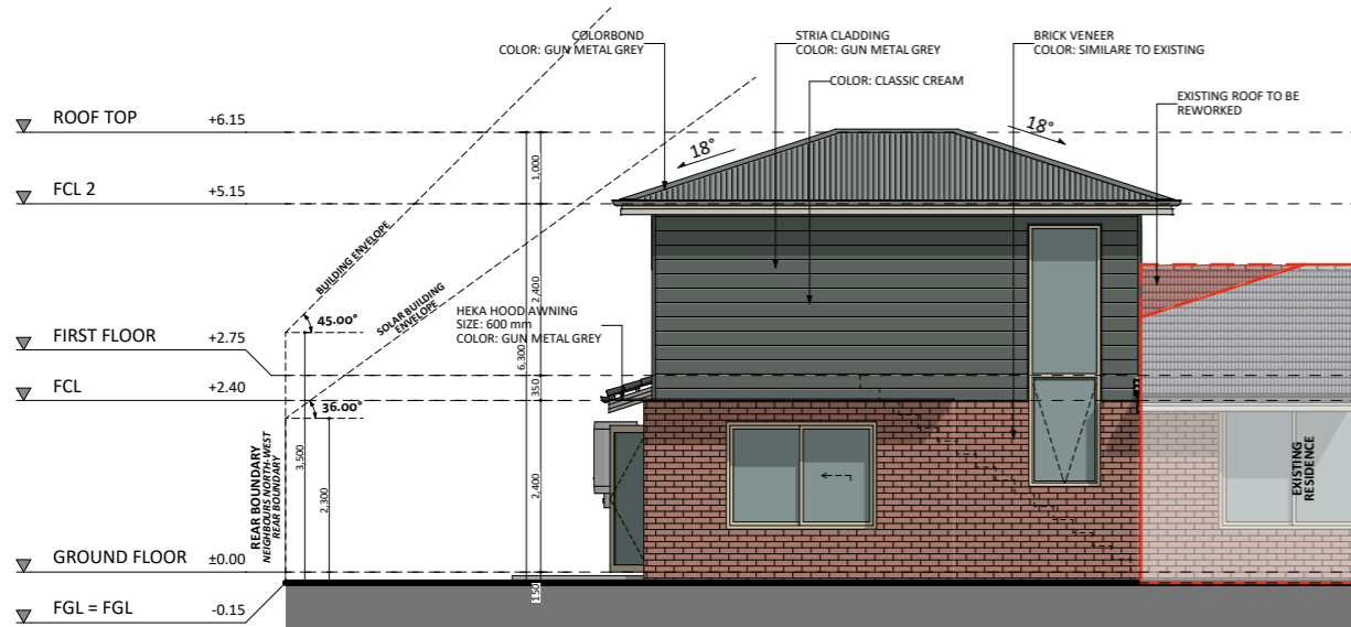
NORTH-EAST
