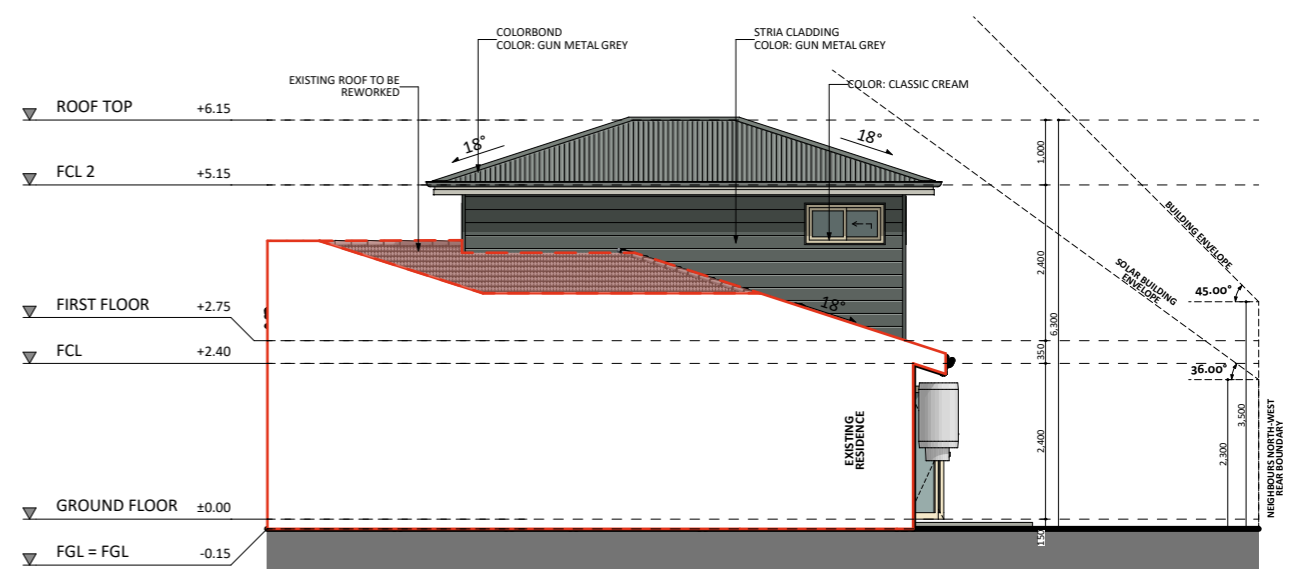
SOUTH-WEST ELEVATION
