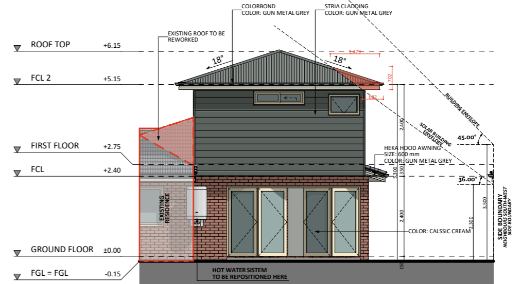
SOUTH-EAST ELEVATION
