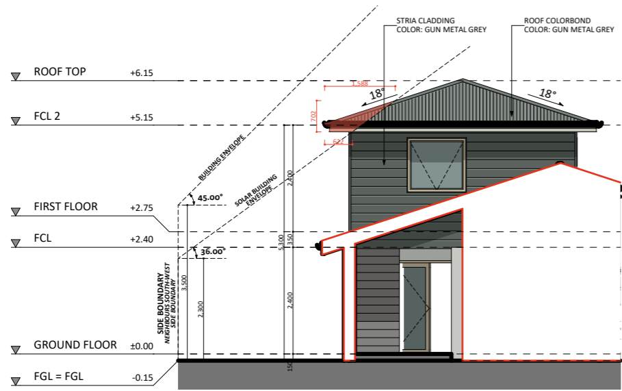
NORTH-WEST ELEVATION
