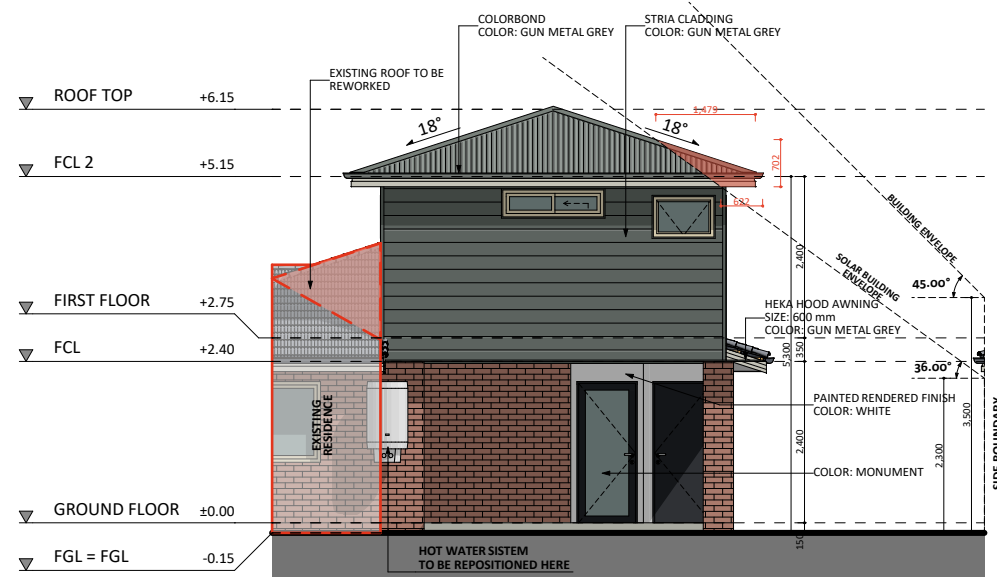
SOUTH-EAST ELEVATION
