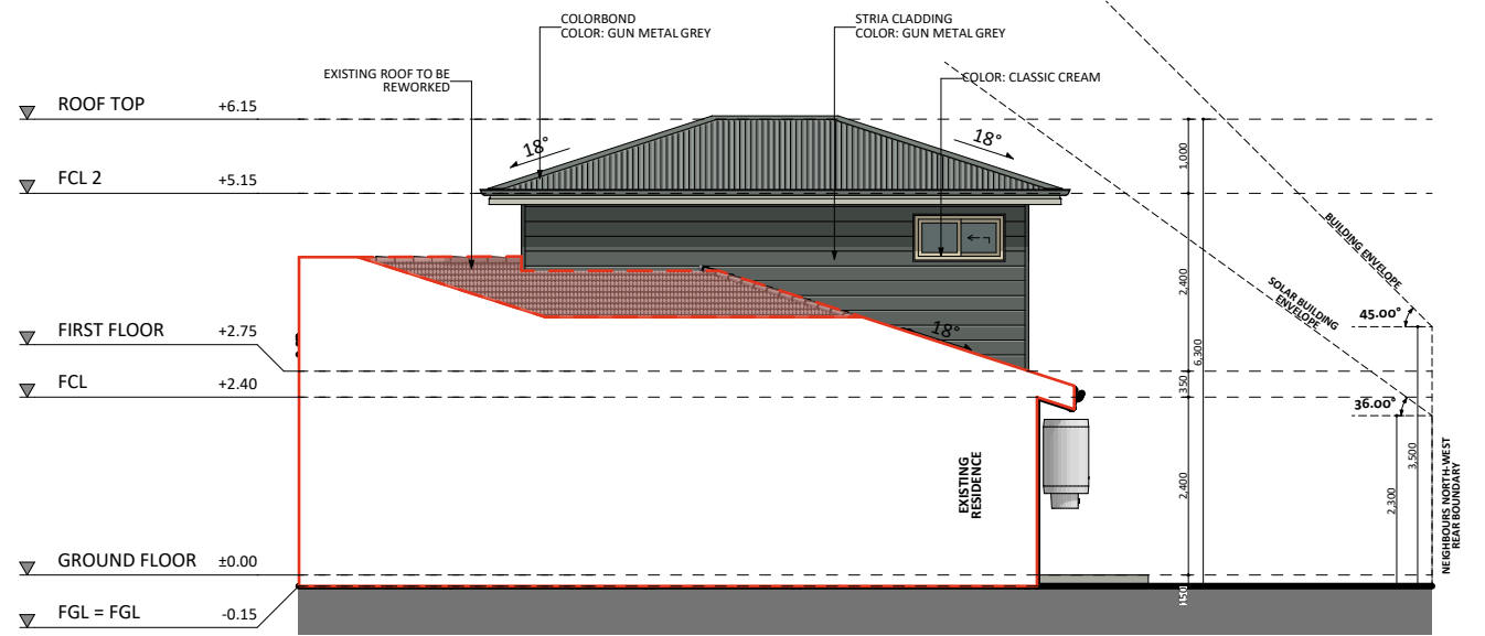
SOUTH-WEST ELEVATION
