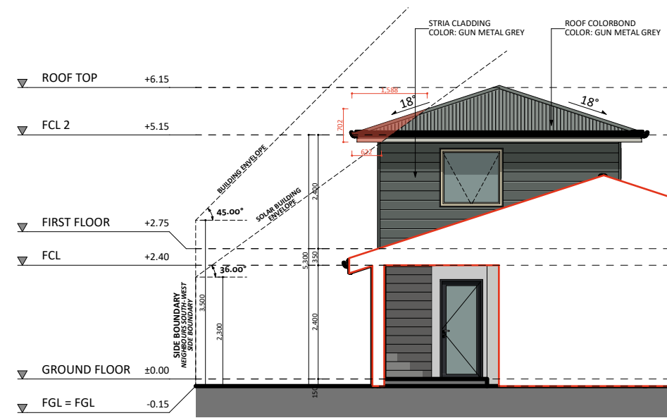
NORTH-WEST ELEVATION
