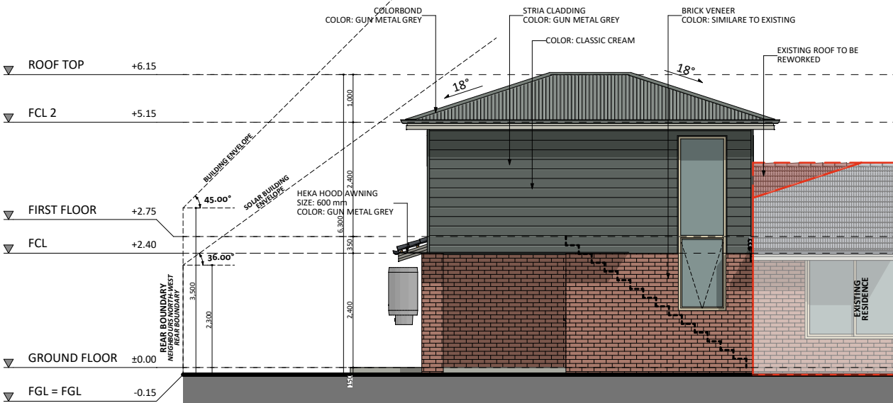
NORTH-EAST ELEVATION
