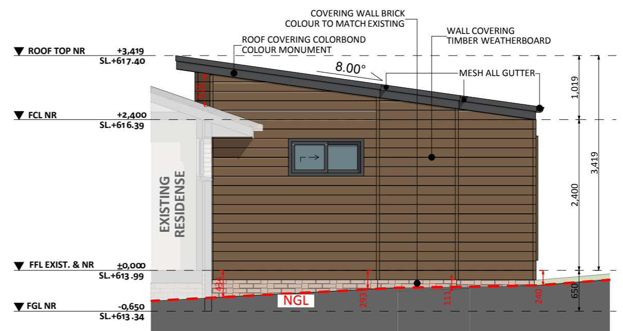
ELEVATION 03
