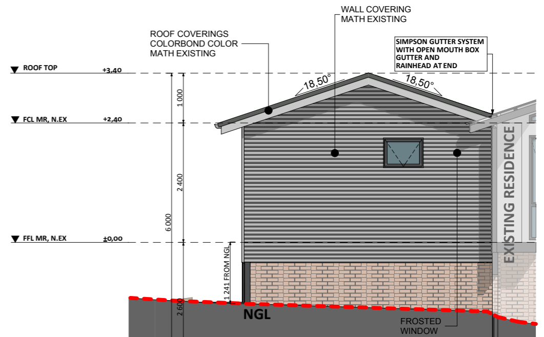
SOUTH ELEVATION
