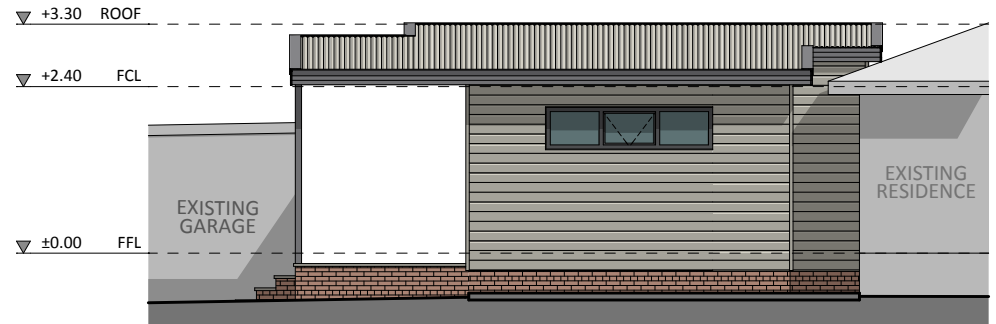
ELEVATION 03
