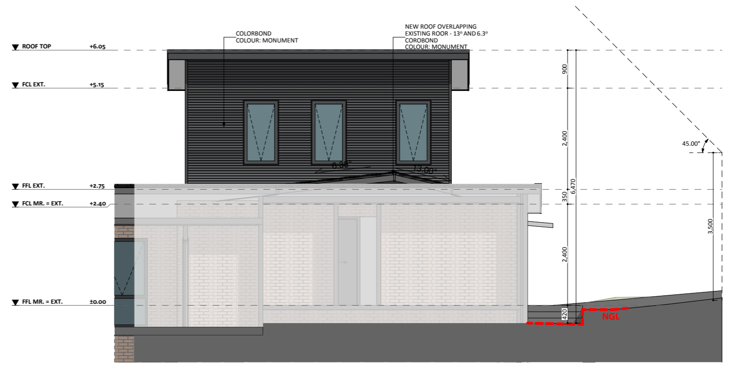
NORTH ELEV.
