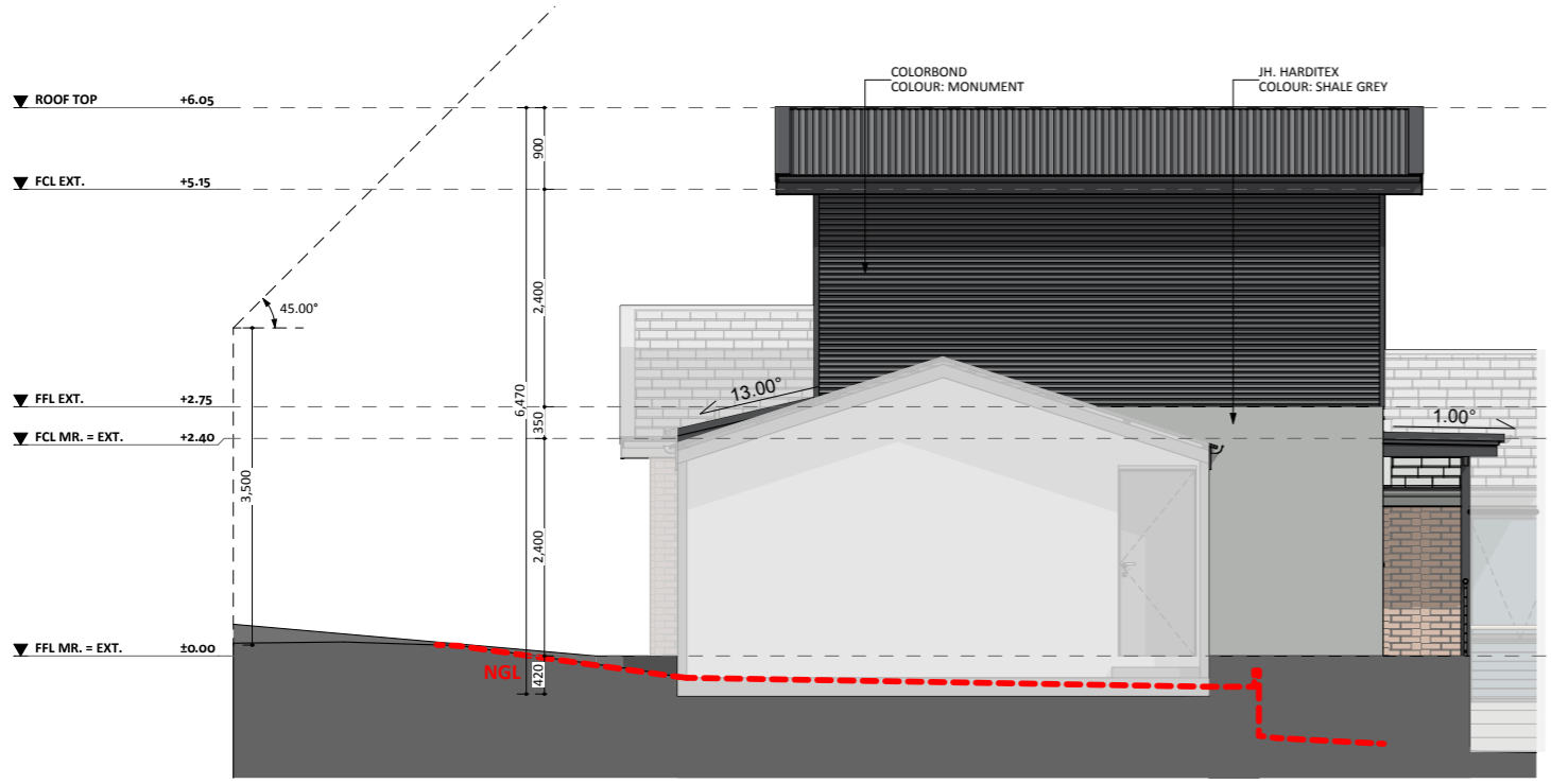
SOUTH ELEV.
