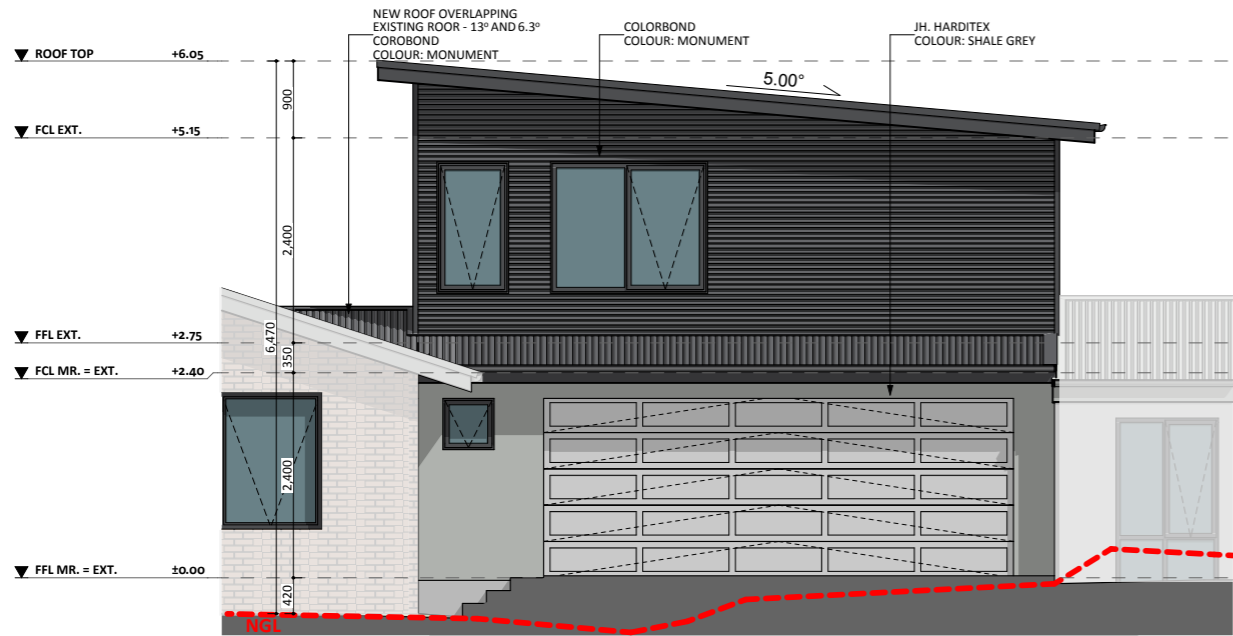
WEST ELEV.
