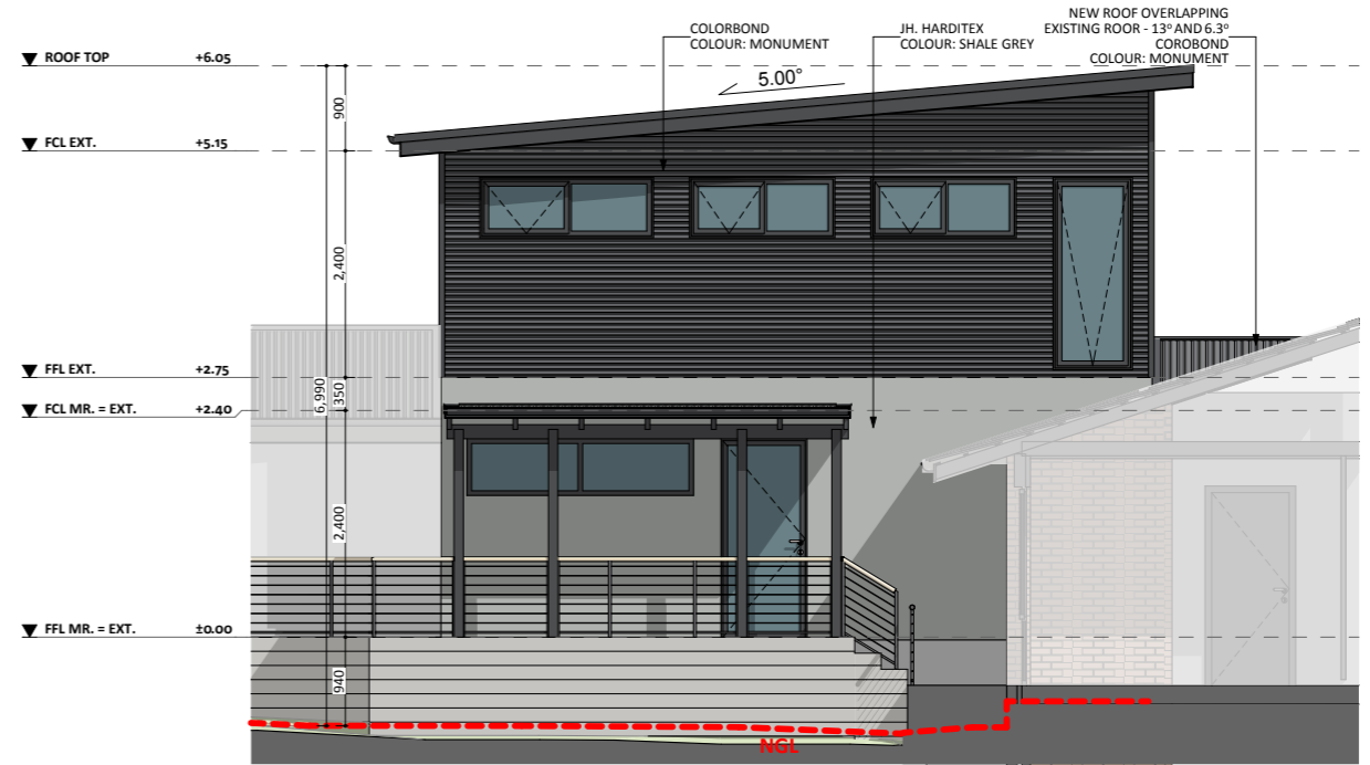
EAST ELEV.
