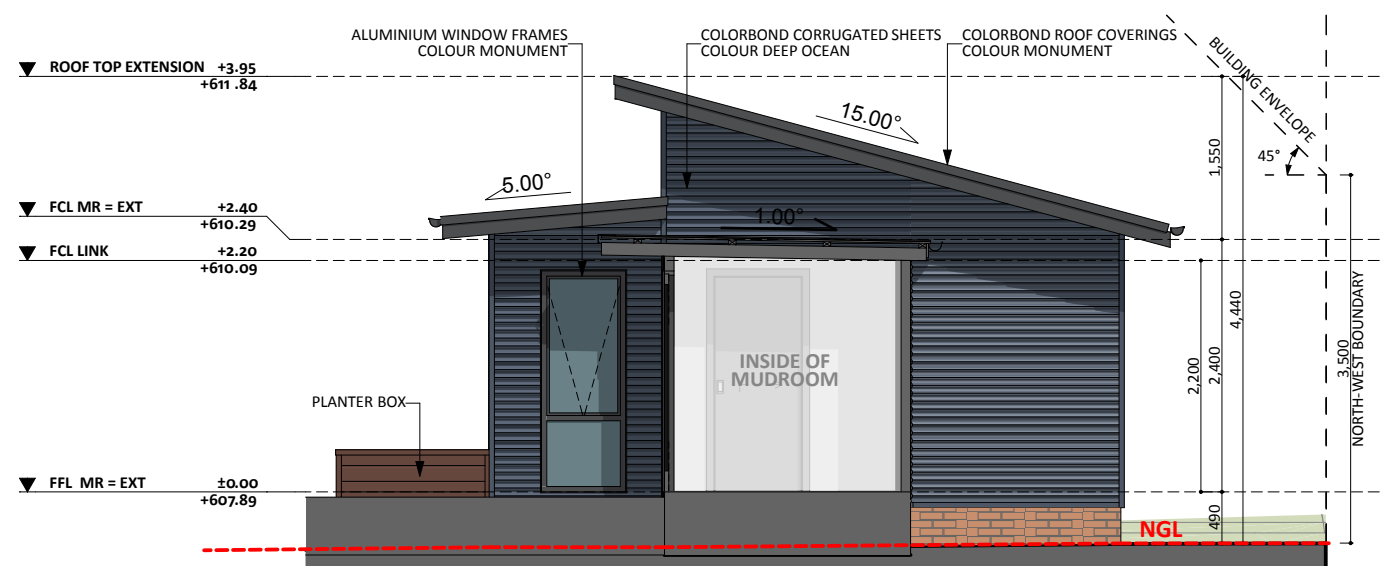
NORHT-EAST ELEVATION
