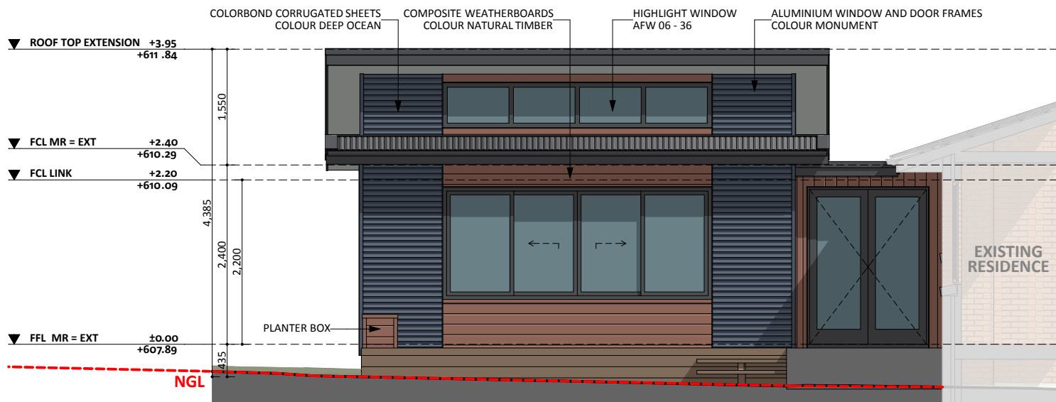
SOUTH-EAST ELEVATION
