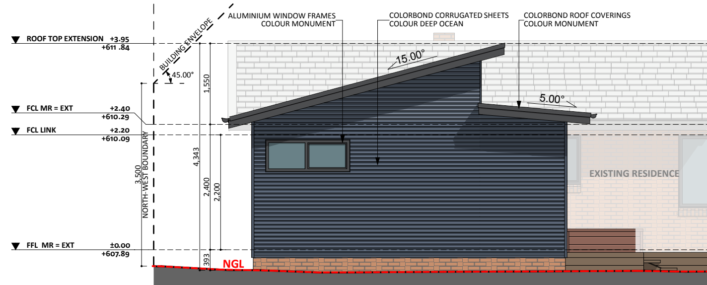
SOUTH-WEST ELEVATION
