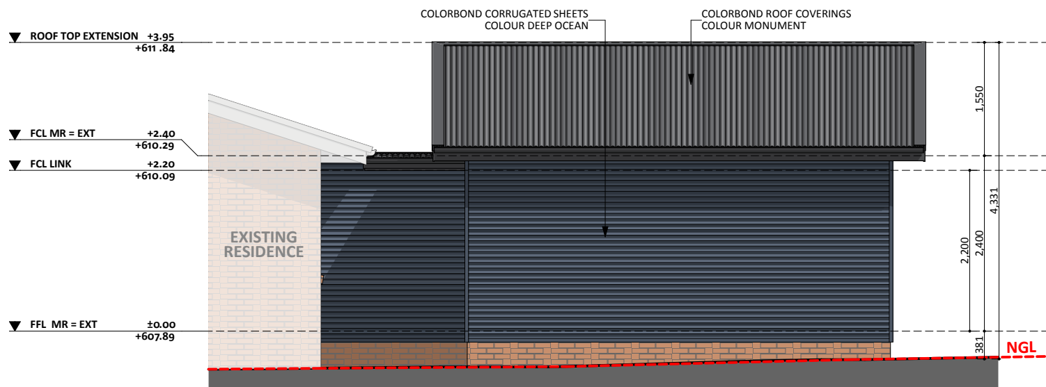
NORTH-WEST ELEVATION
