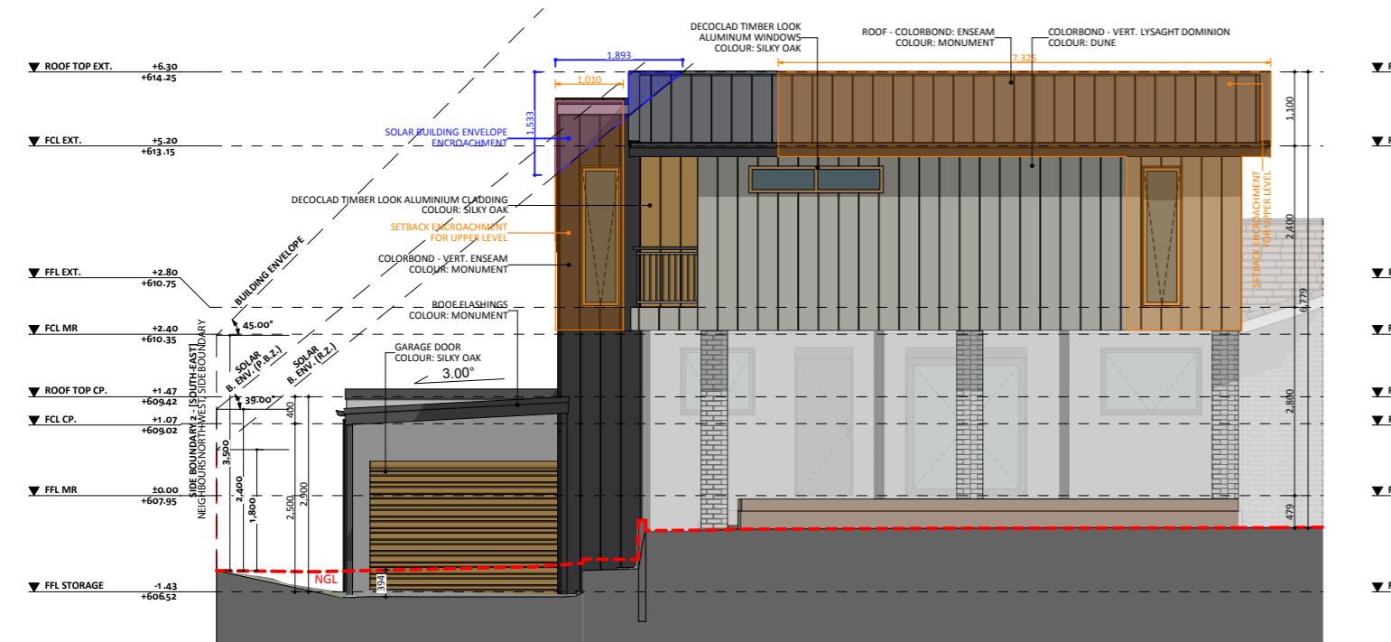
NORTH-EAST ELEVATIONS
