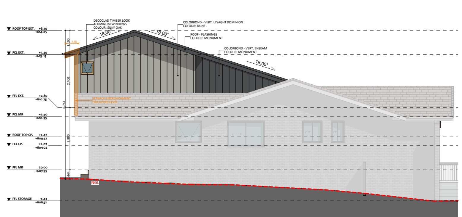
NORTH-WEST ELEVATIONS
