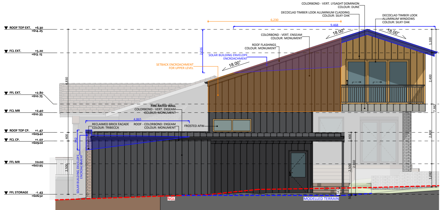
SOUTH-EAST ELEVATIONS
