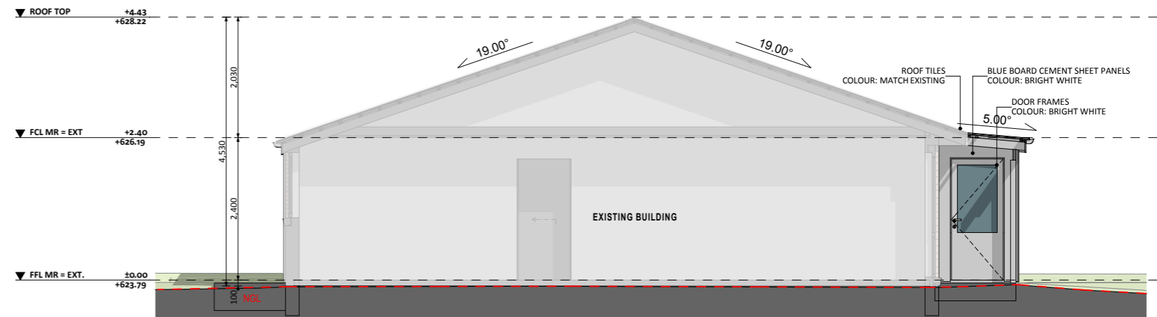
WEST ELEV. - EXT.
