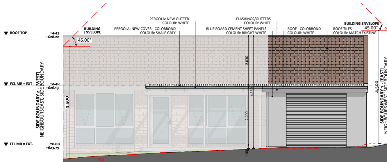
SOUTH ELEV. - EXT.
