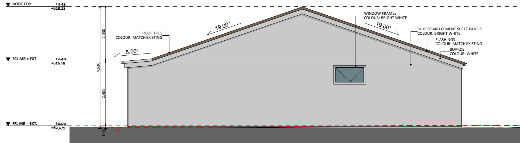
EAST ELEV. - EXT.
