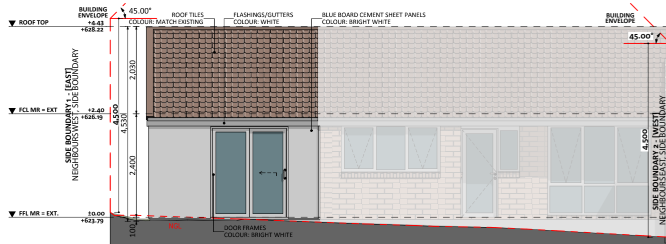
NORTH ELEV. - EXT.
