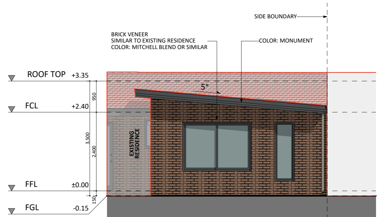
SOUTH-EAST ELEVATION
