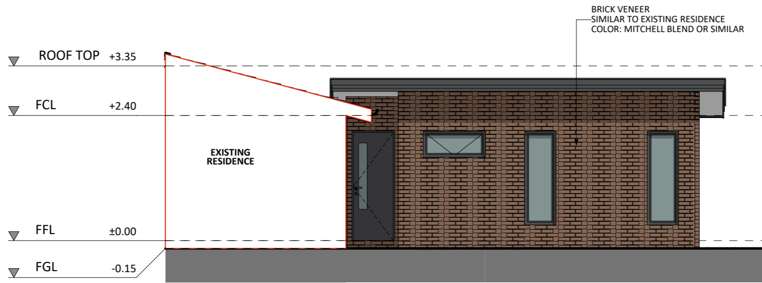
SOUTH-WEST ELEVATION
