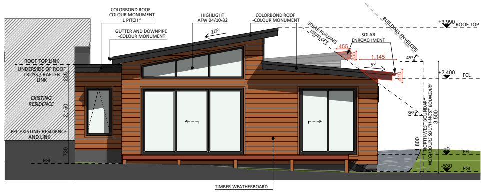
NORTH-EAST ELEVATION
