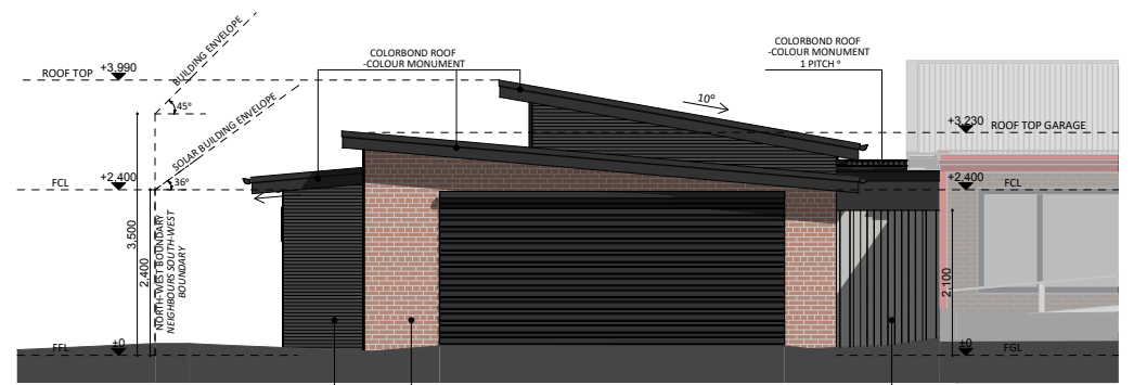
NORTH-EAST ELEVATION
