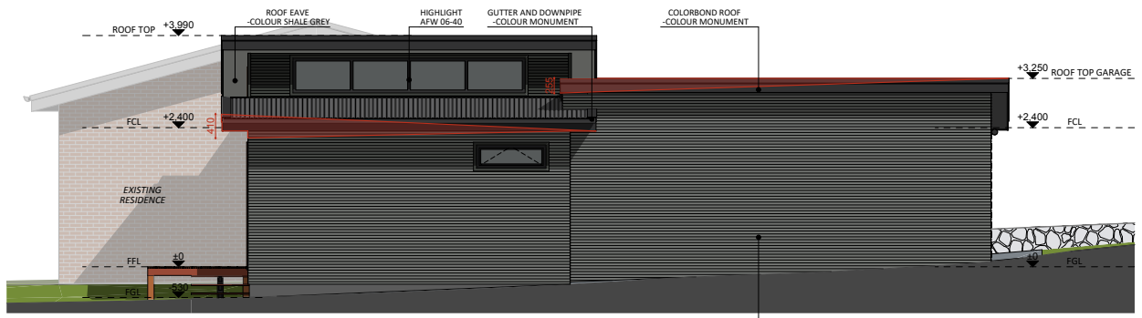
NORTH-WEST ELEVATION
