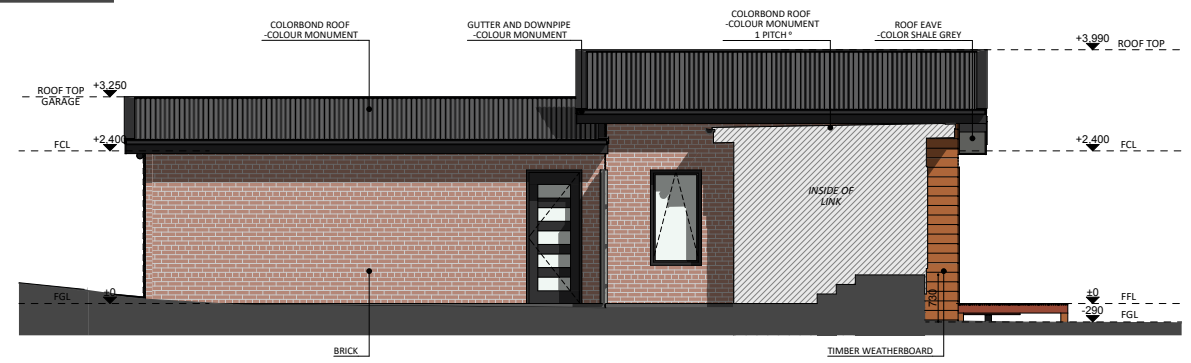
NORTH-WEST ELEVATION
