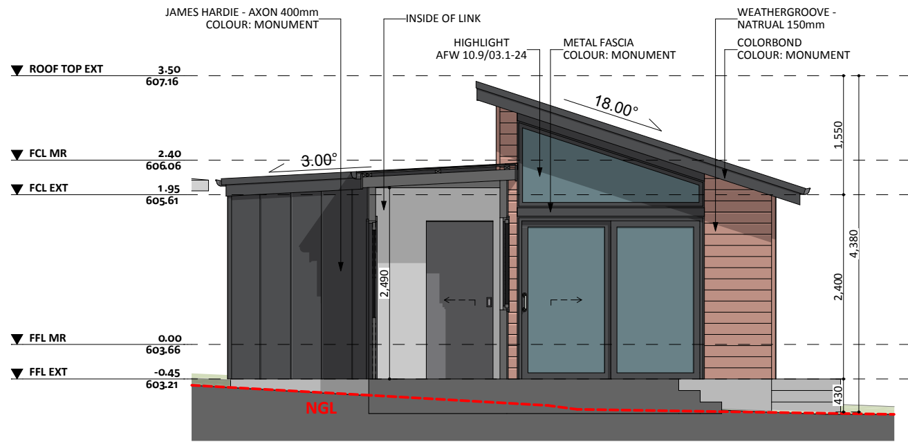
NORTH-WEST ELEV.
