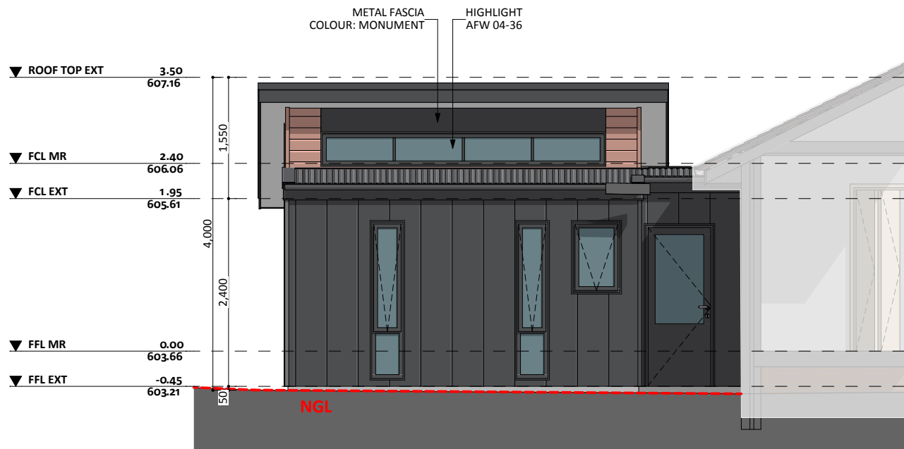
NORTH-EAST ELEV.
