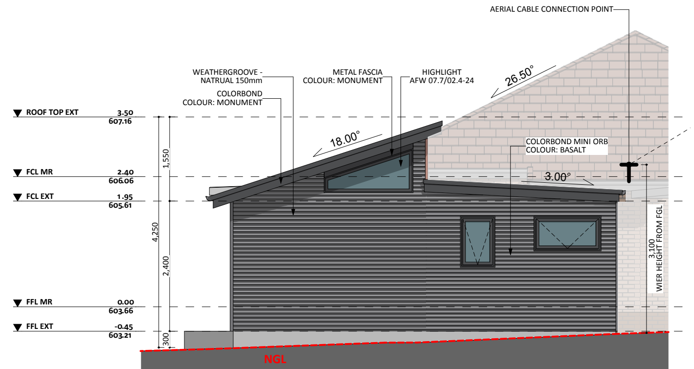
SOUTH-EAST ELEV.
