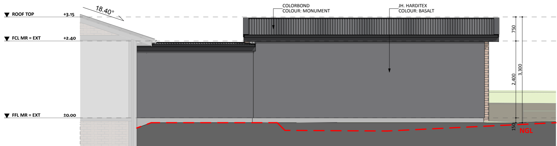
ELEVATION 03
