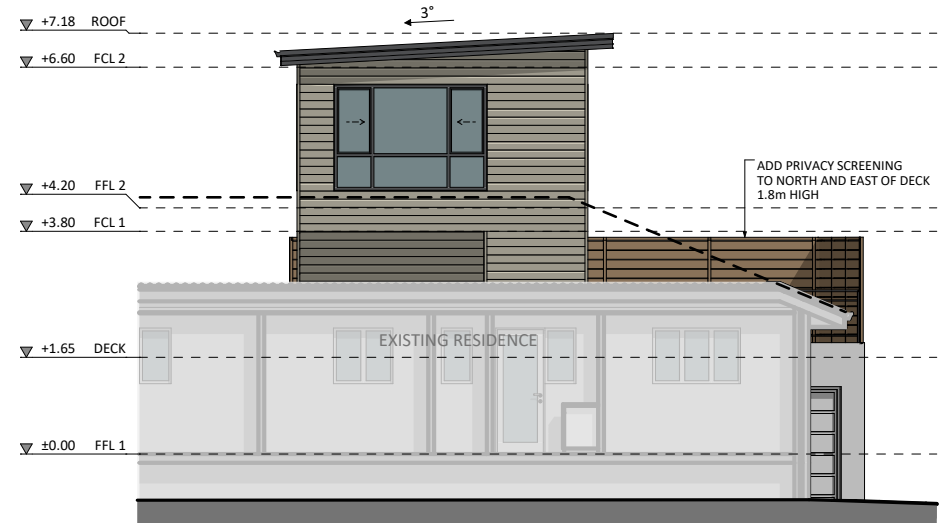
SOUTH ELEVATION
