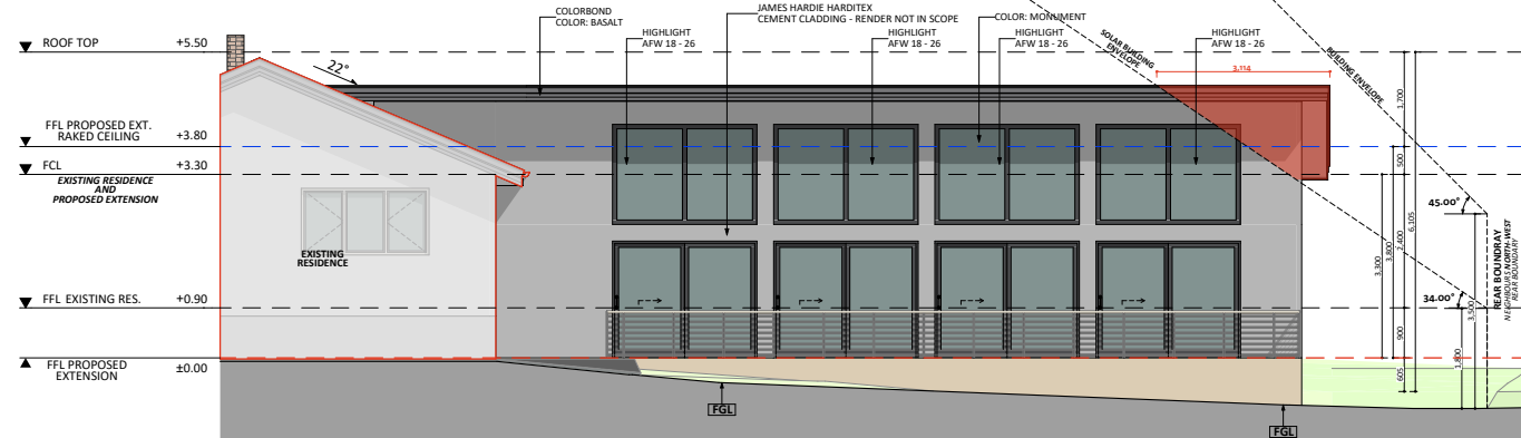
NORTH-EAST ELEVATION
