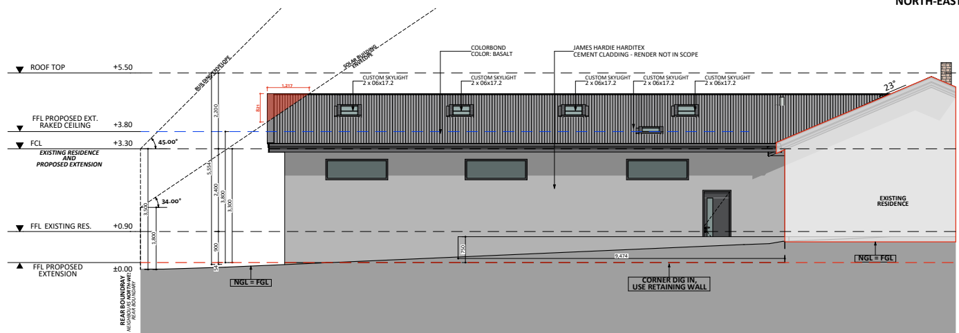
SOUTH-WEST ELEVATION
