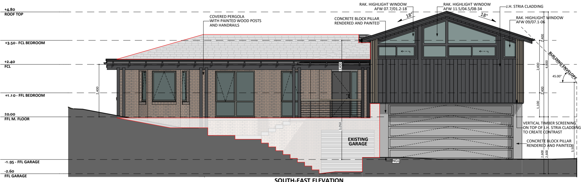
SOUTH-EAST ELEVATION
