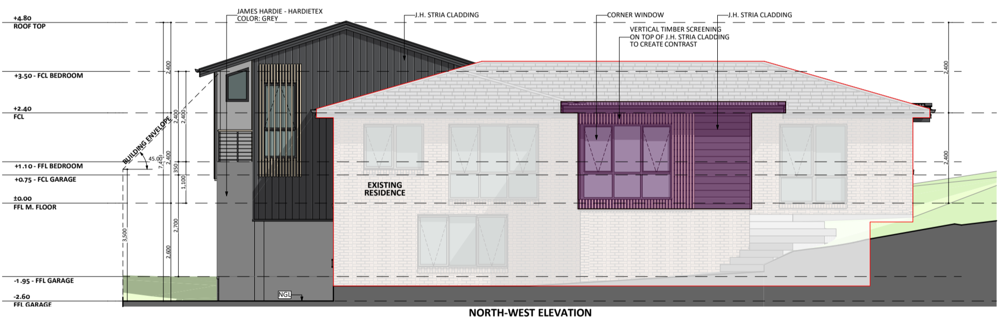
NORTH-WEST ELEVATION
