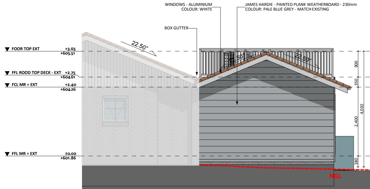
ELEVATION 03
