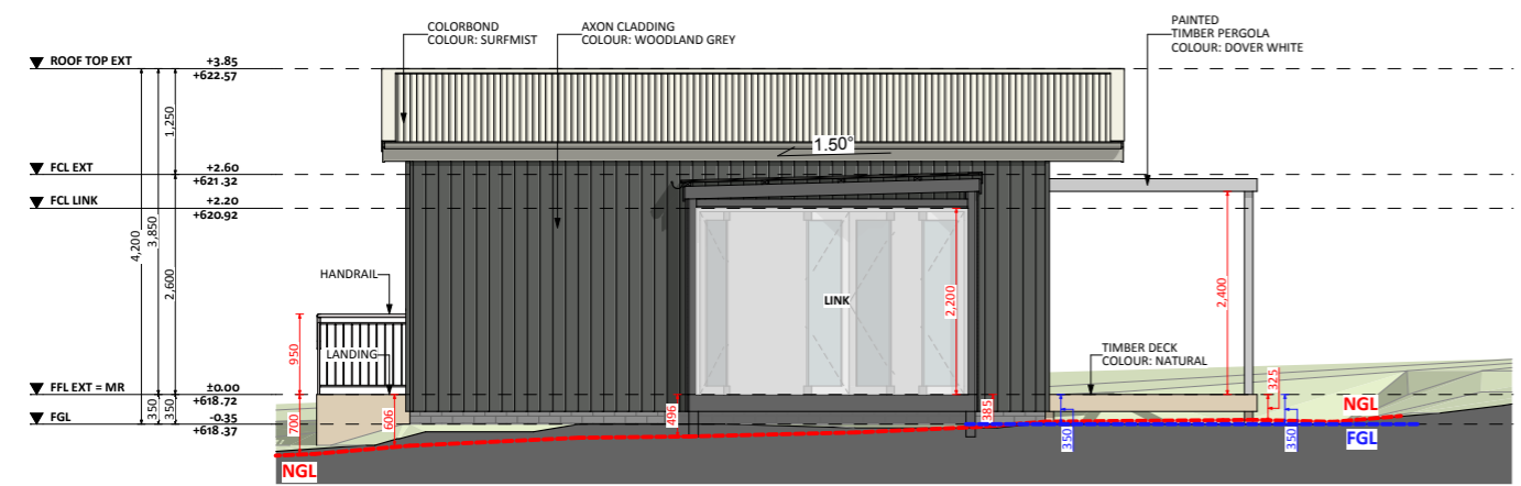
ELEVATION 03
